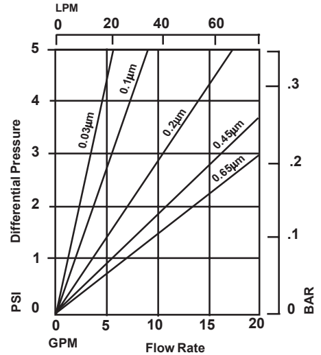
Polyethersulfone Cartridges: Flow rate vs. ΔP for a 1 cps liquid @ 73°F (23°C)**
